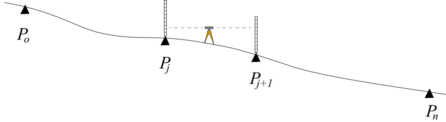
Figure 2.2: A single leveling run from point P_0 to point P_n ; courtesy Michael Bevis
