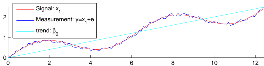
Figure 17.1: Sinusoidal signal containing random noise and linear trend
