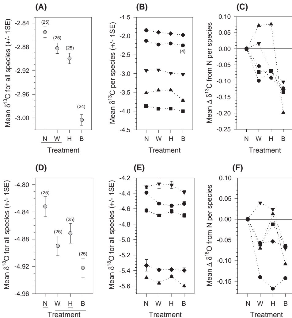
Fig. 2. Experiment #1, Pre-treatment of bulk skeletal samples below the tissue layer from five species of coral: Pavona clavus (◆), Porites lobata (●), Montipora verrucosa (▼), Pavona gigantea (▲), and Porites compressa (■). Pre-treatments were: N=no pre-treatment, W=water pre-treatment, H=H 2 O 2 pre-treatment, B=bleach pre-treatment. (A) and (D) Overall mean \delta^{13}\text{C} and \delta^{18}\text{O} for all species, respectively. Within each panel, treatment labels along the x-axis that share a line indicate that the means do not significantly differ from each other. (B) and (E) Mean \delta^{13}\text{C} and \delta^{18}\text{O} for each treatment within each species, respectively. In (B), error bars are always smaller than the symbols. (C) and (F) Mean change in \delta^{13}\text{C} ( \Delta\delta^{13}\text{C} ) and in \delta^{18}\text{O} ( \Delta\delta^{18}\text{O} ) from no pre-treatment for each species, respectively. SE=standard error of the mean, the sample size of each mean is 5 except where indicated. Statistics given in Table 3.
